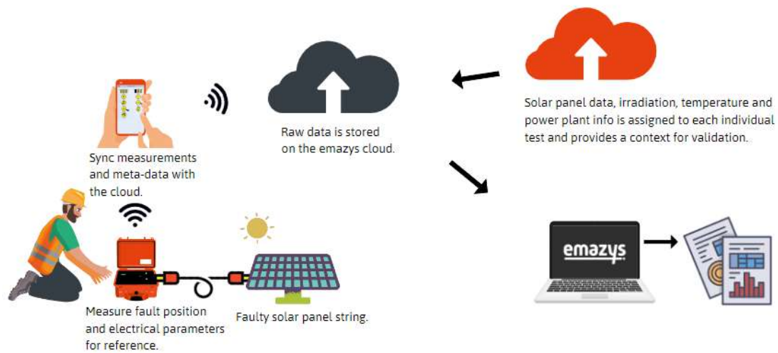
Figure 5: An illustration showing an overview of the field test work flow with use of the android app and web app cloud.
