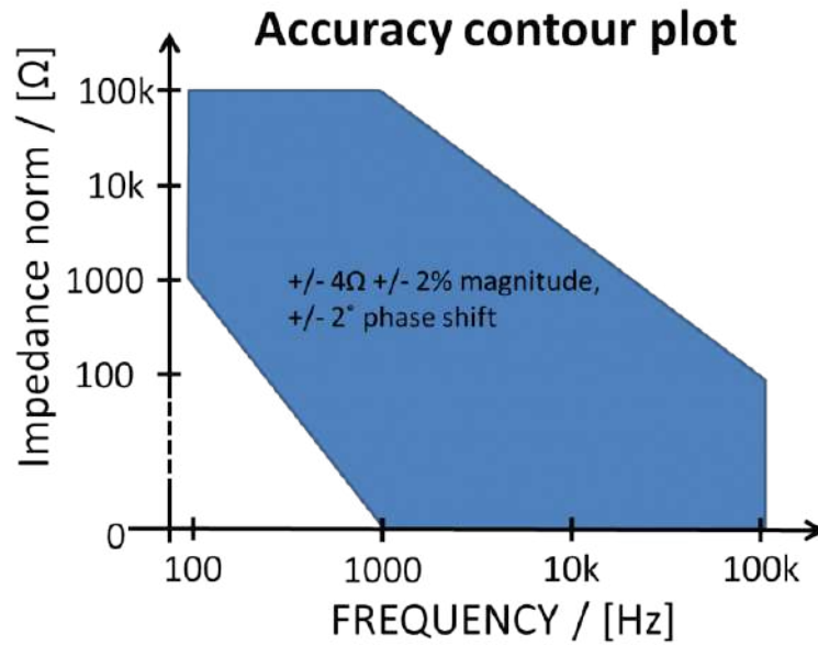
Figure 6: In this graph we see the impedance accuracy contour plot for the Z200 PV Analyzer.
