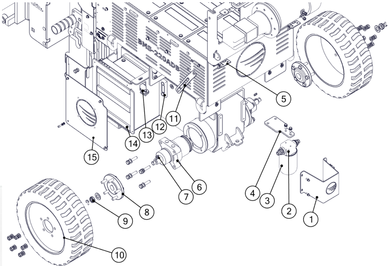
Fig. 03 Rear wheel & Oil filter
