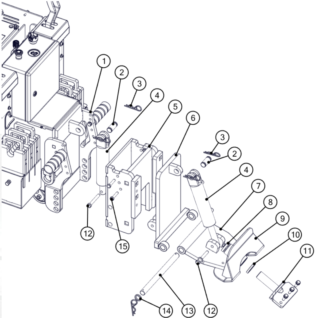
Fig. 02 Cutting head
